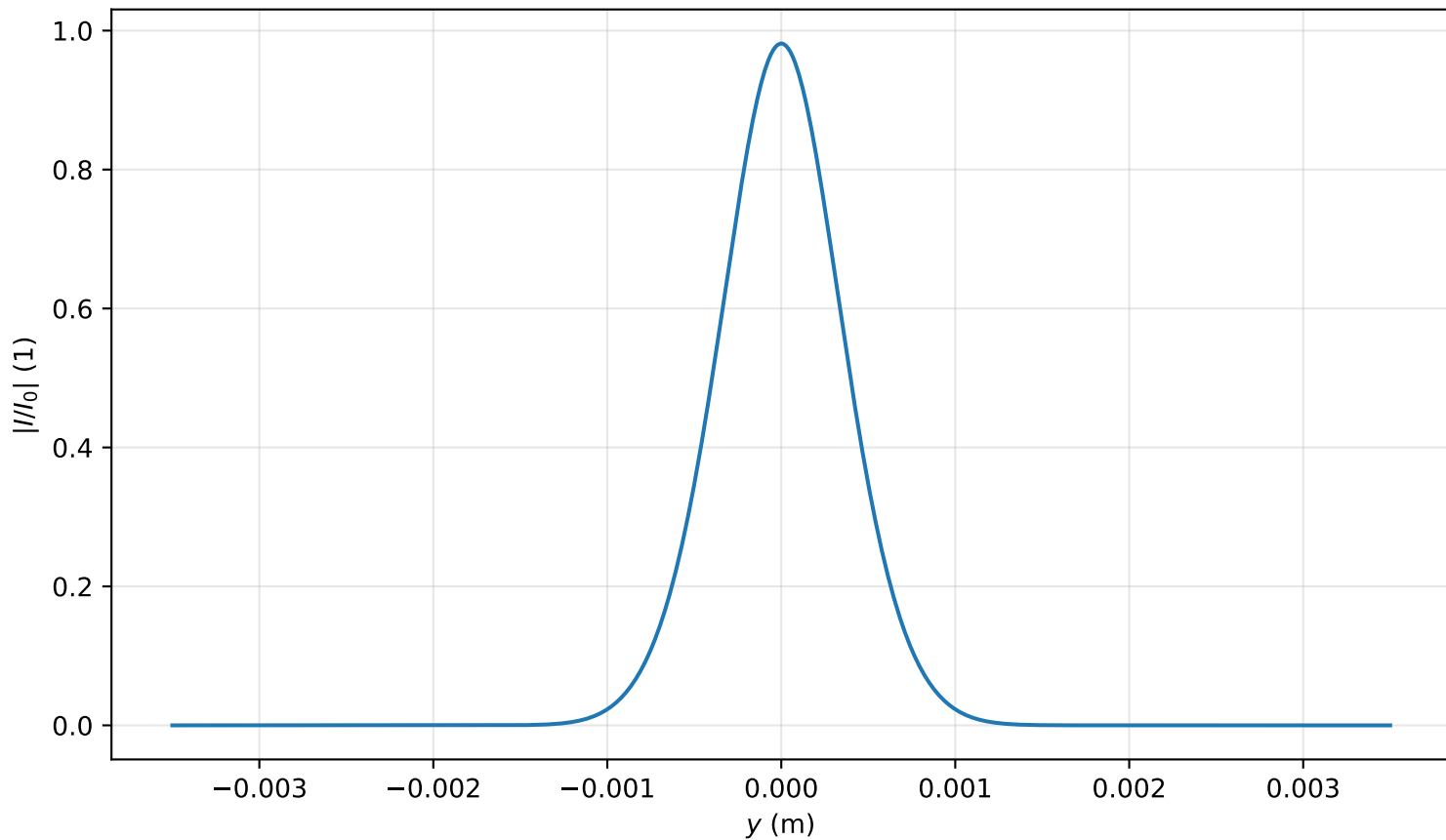
Intensity profile I(x=0, y, z=0.716)/I_0 , P_{in}=0.3P_{cr} , artificial time
